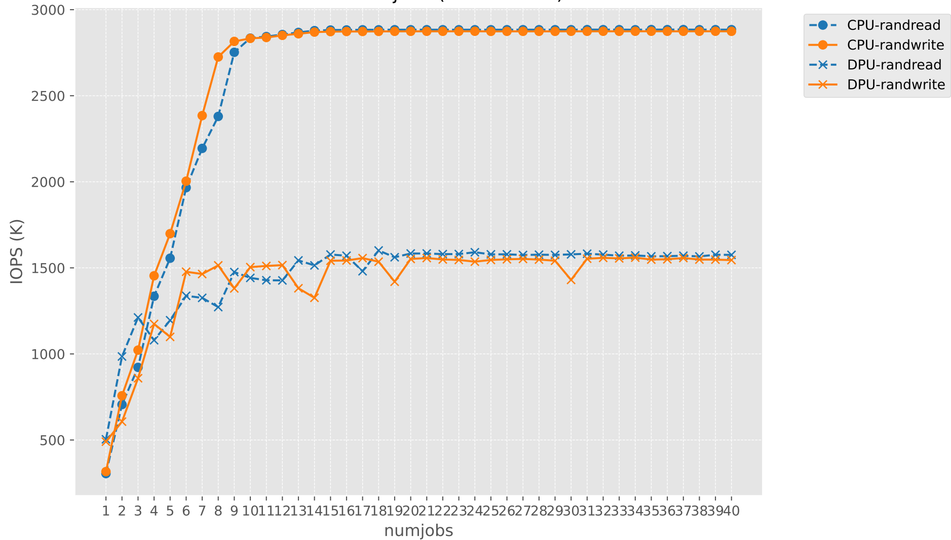
IOPS vs numjobs (CPU vs DPU)
